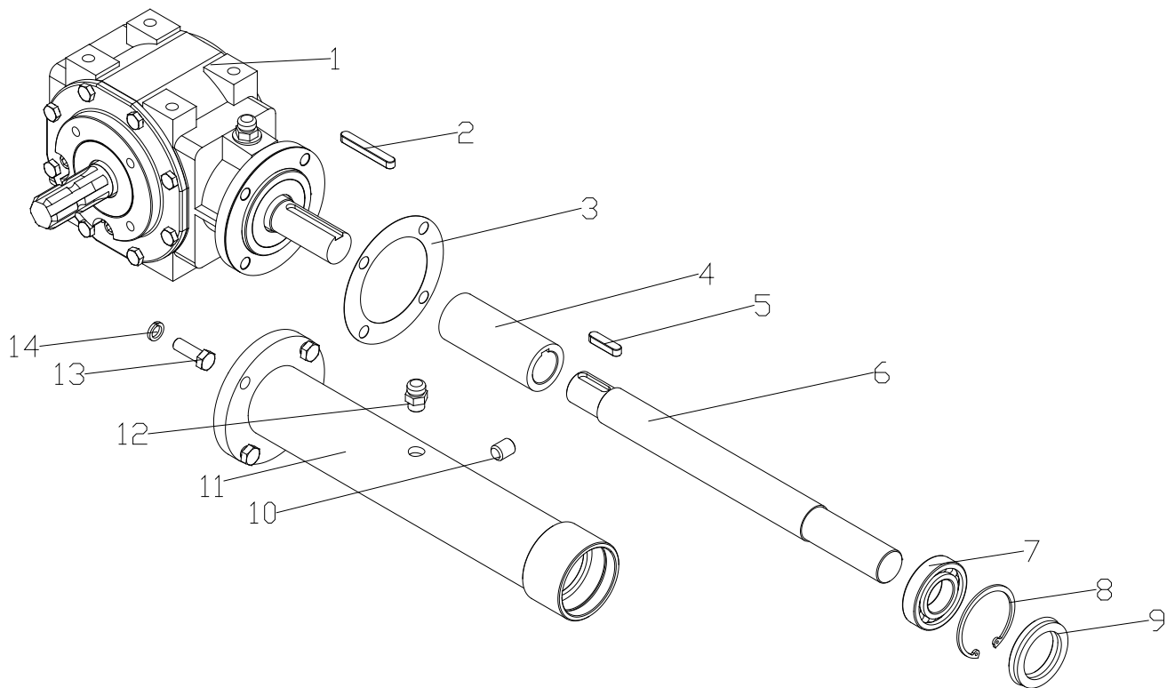
Fig. 3 Gearbox components
