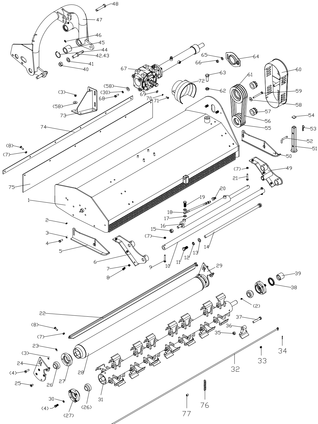
Fig. 1 Main mower
